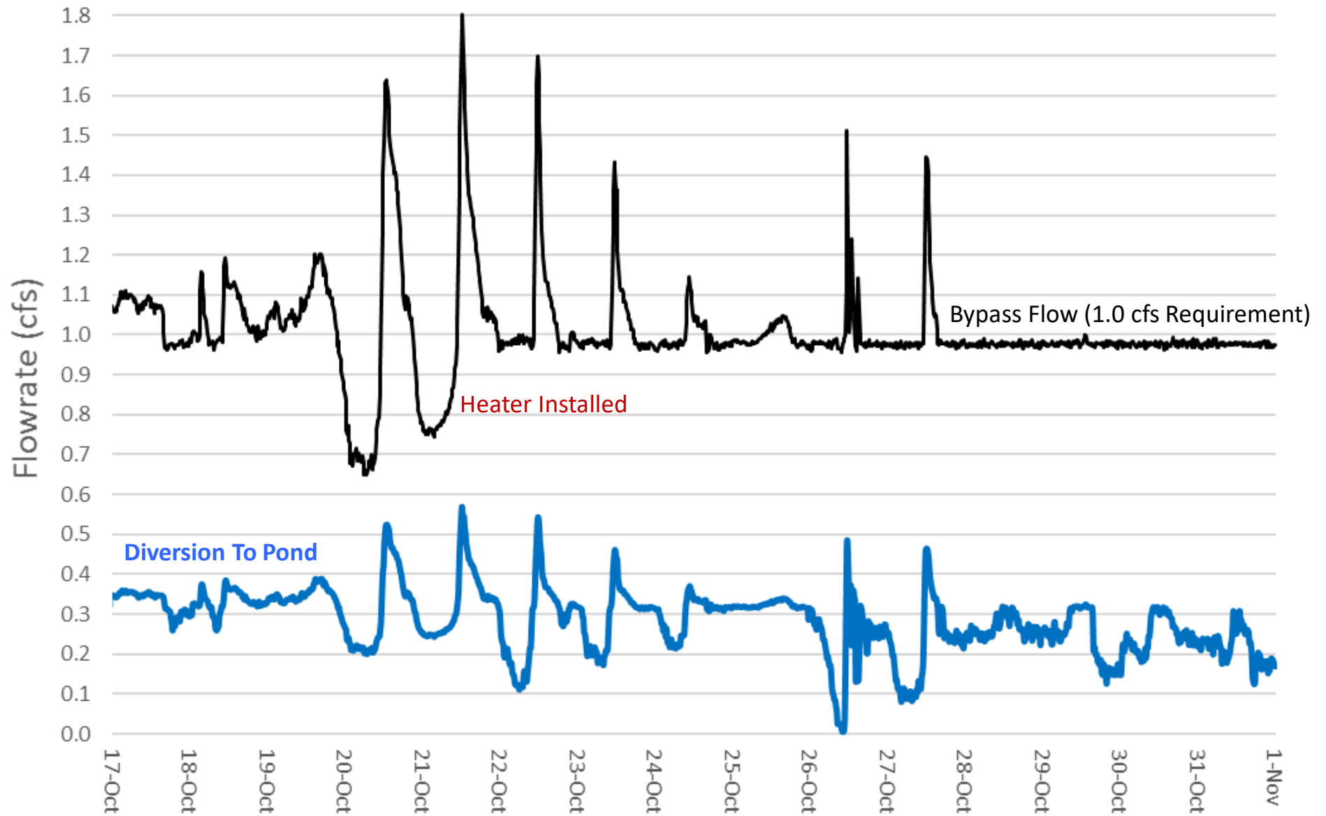
A-Basin Snowmaking Diversion (Automated Weir set to 1.0 cfs Bypass)
