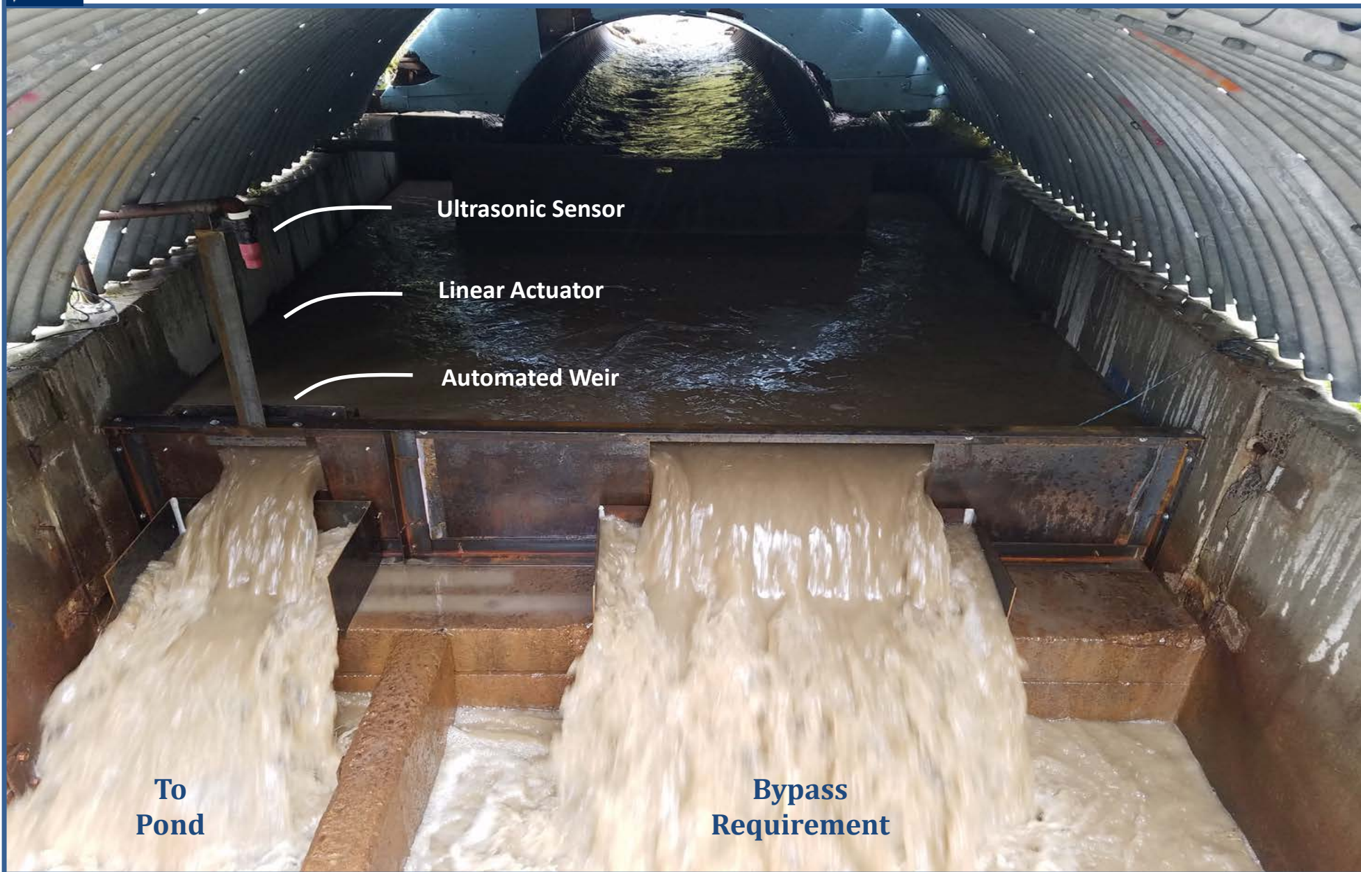
Figure 1 A-Basin Snowmaking – Automated Diversion Structure
