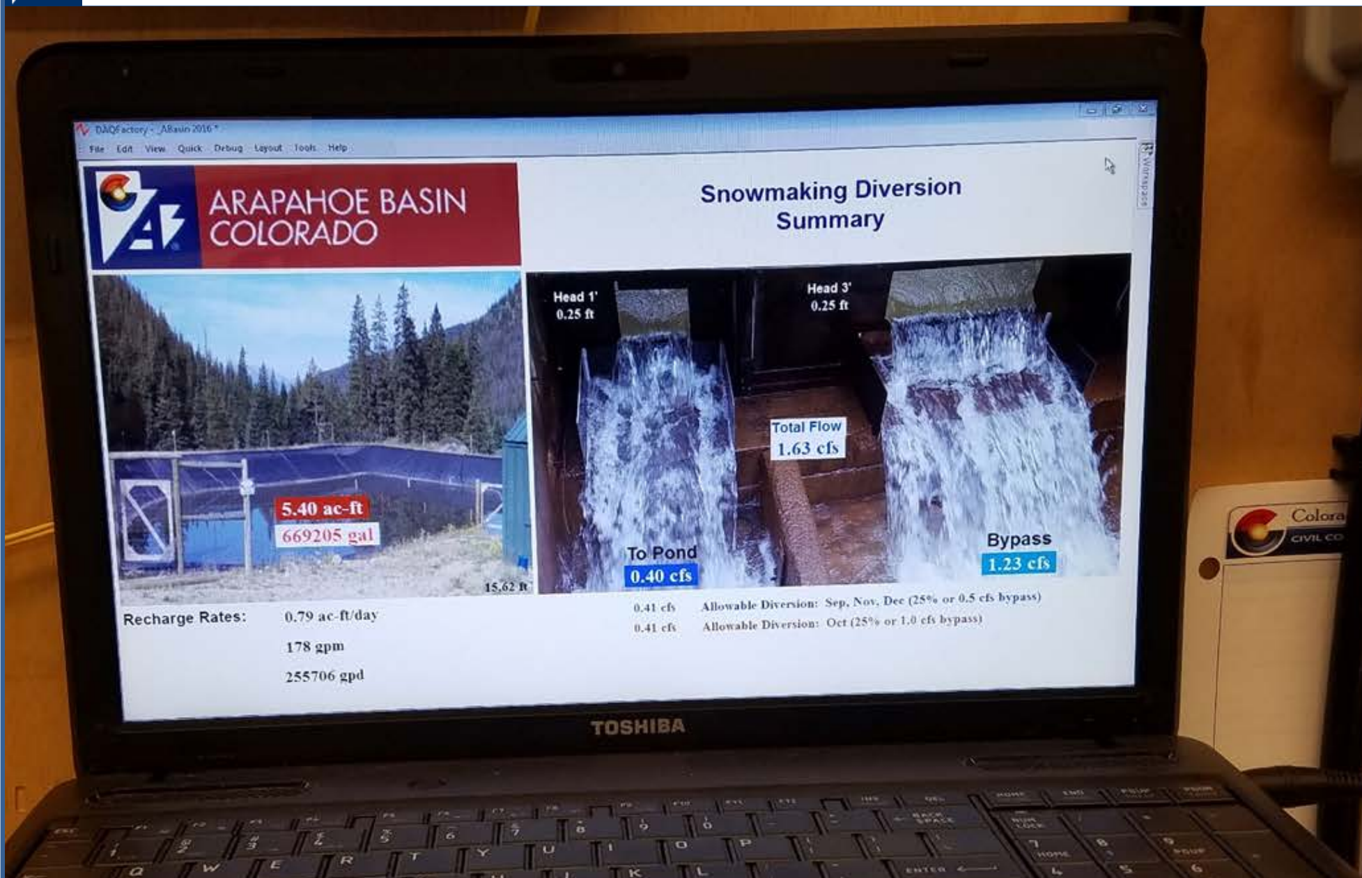
A-Basin Snowmaking Computer – Remote Connection Screenshot (Labjack, DAQFactory)
